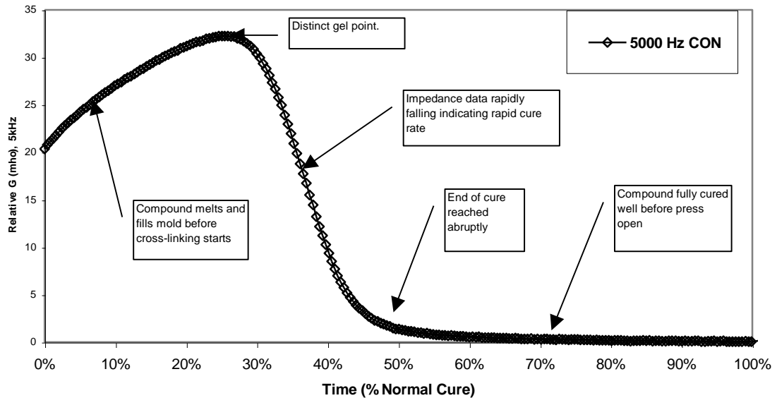
Figure 11: Compound 2 Impedance Signatures
