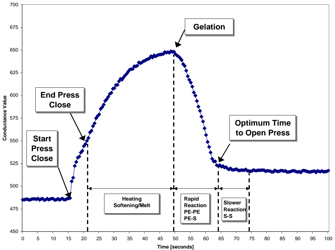
Figure 3: Typical SMC Impedance Signature
