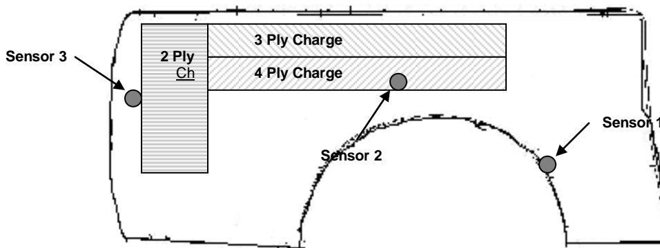
Figure 6: Relative Locations of Sensors and Charge Pattern
