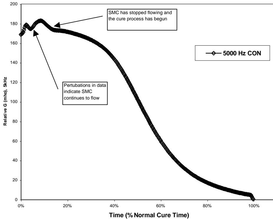
Figure 9: Impedance Signature Showing Poor SMC Flow
