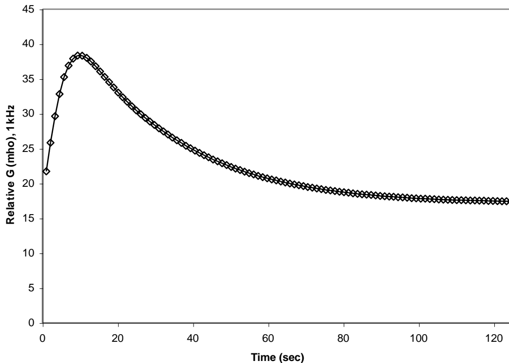
Figure 14: Typical Phenolic Impedance Signature
