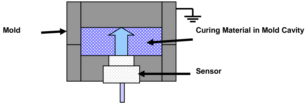
Figure 1: Capacitor formed by mold/sensor arrangement
