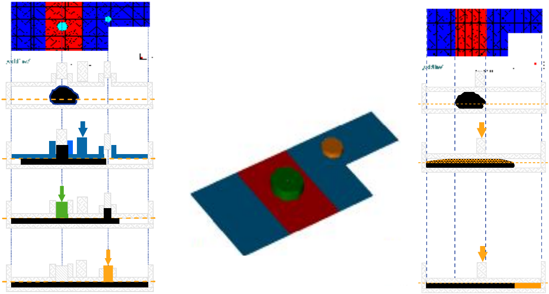
Figure 6 shows a compression mould built for the DCM process on the left as opposed to a conventional tool (process) on the right
